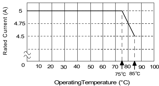
DLW5BSM191SQ2 Temperature Derating
